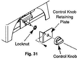
Control Knob
